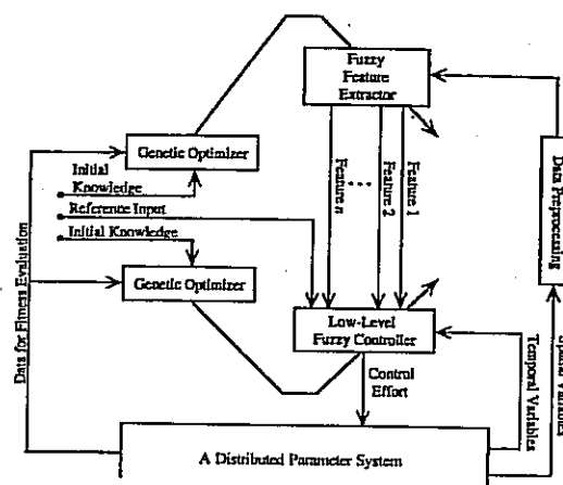
Figure 4: GA-Based Learning Hierarchical Control Architecture
