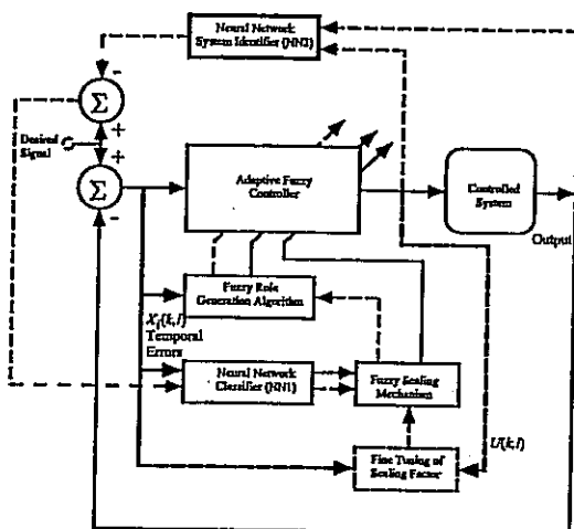
Figure 1: Block Diagram of the Adaptive Neuro-Fuzzy Controller
