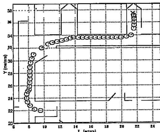
Figure 7: Goal-seeking navigation using fuzzy-behaviors.
