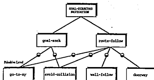
Figure 6: Hierarchical decomposition of mobile robot behavior.
